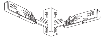
L - Coupler Inside/outside (converts)
