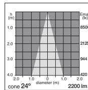
100w QR-LP111 24° lamp
