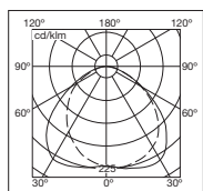
DLOR = 0.64 32w
