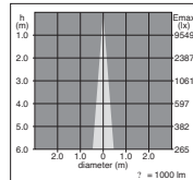
50w 10° Spot
