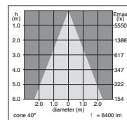
cone 40° 70w NB
