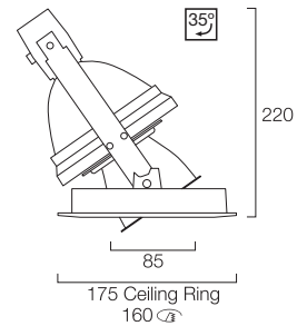
Double Focus Adjustable
