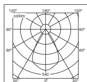
DLOR = 0.45 100w WB
