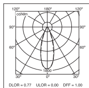
Suspended Lyteframe See page 167
