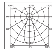
70w 11° Spot 70w 39° Flood
