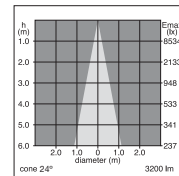
35w CDM-R111 24° lamp
