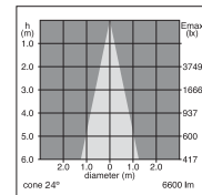
70w CDM-R111 24° lamp
