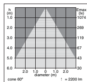
cone 60° 100w WB
