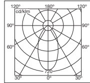
DLOR = 0.71 150w WB
