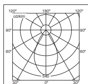
DLOR = 0.43 35w WB
