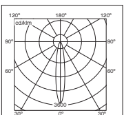
DLOR = 0.61 70w Gimbal
