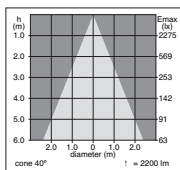
cone 40° 100w NB
