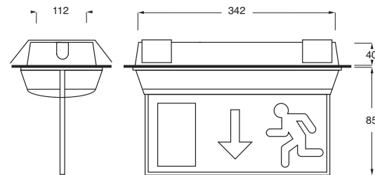
Cut-out size 343 x 116
