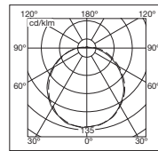
DLOR = 0.41 38w Standard
