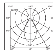
DLOR = 0.38 70w WB
