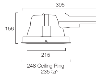
Axial Reflector with Silver Bezel Accessory
