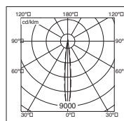
35w 10° Spot 35w 37° Flood
