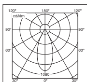
DLOR = 0.51 35w NB
