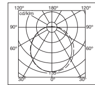
DLOR = 0.40 38w 3 Bar Grille
