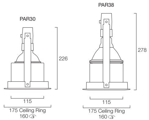
PAR30 Deep Multigroove Darklight
