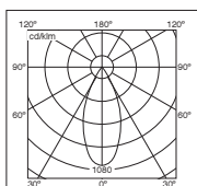
DLOR = 0.55 100w NB
