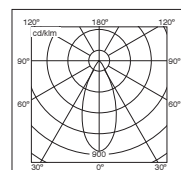
DLOR = 0.46 70w NB
