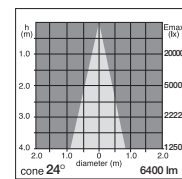
70w HIPAR111 24° lamp
