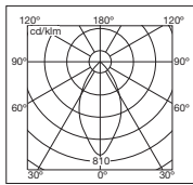
35w 60° Flood
