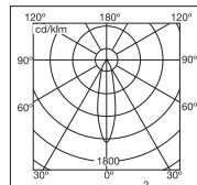
DLOR = 0.40 100w
