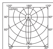
DLOR = 0.67 150w Gimbal
