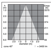
cone 40° 35w NB
