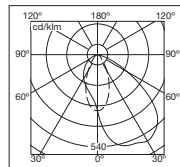
DLOR = 0.62 150w W/W
